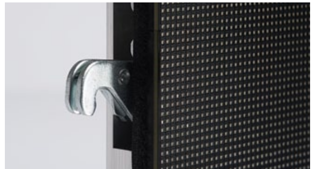
▲ Innovative locking mechanism 1 provides a truly seamless display and easy setup and servicing
